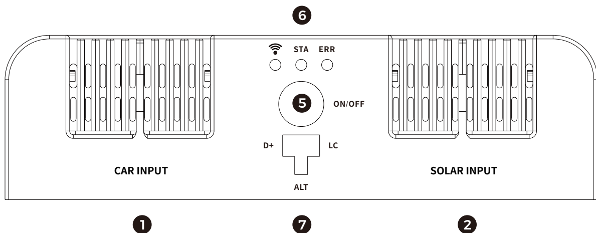
Figure 1 Front Panel
